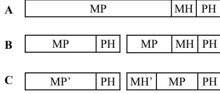
Figure 6. Message-packet alignment
