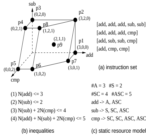
Figure 4.4. Verifying an instruction set having no SRM
