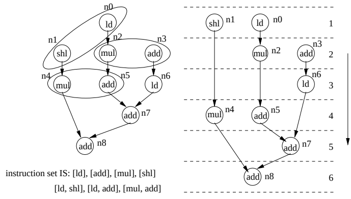
Figure 1.1. Instruction selection prior to scheduling may yield inferior results
