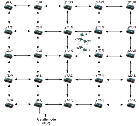
Fig. 5. A 5 \times 5 node static wireless sensor network with one mobile cluster including 5 cluster nodes.
