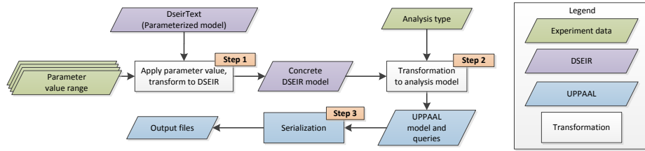
Fig. 3: Octopus example transformation orchestration
