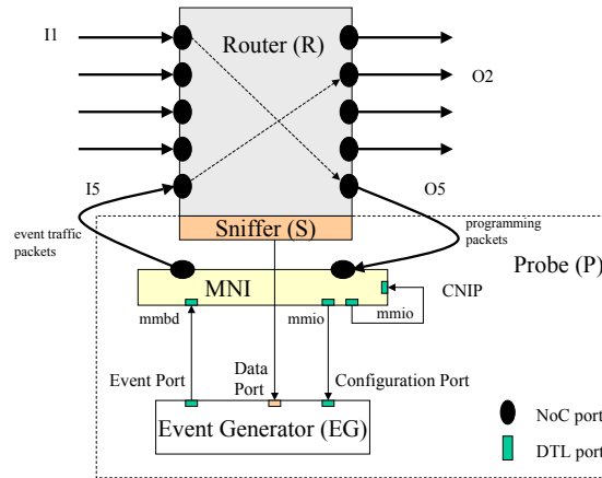
Fig. 4. \mathcal{A} etheral Probe Architecture
