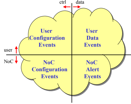
Fig. 3. NoC Event Space
