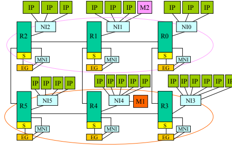
Fig. 8. NoC2 extended with probes, distributed service
