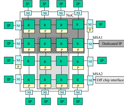
Fig. 2. Distributed Monitoring Service
