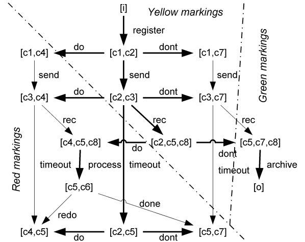
FIGURE 13. The OG of S_1 partitioned for non-live sequences
