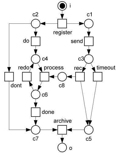
FIGURE 2. An example system S for net N
