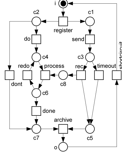
FIGURE 3. The short-circuited system \underline{S} = (\underline{N}, [i])
