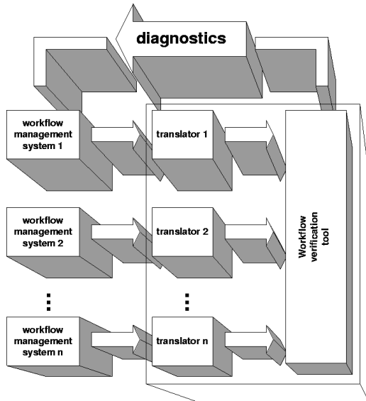
FIGURE 11. The approach supported by Woflan
