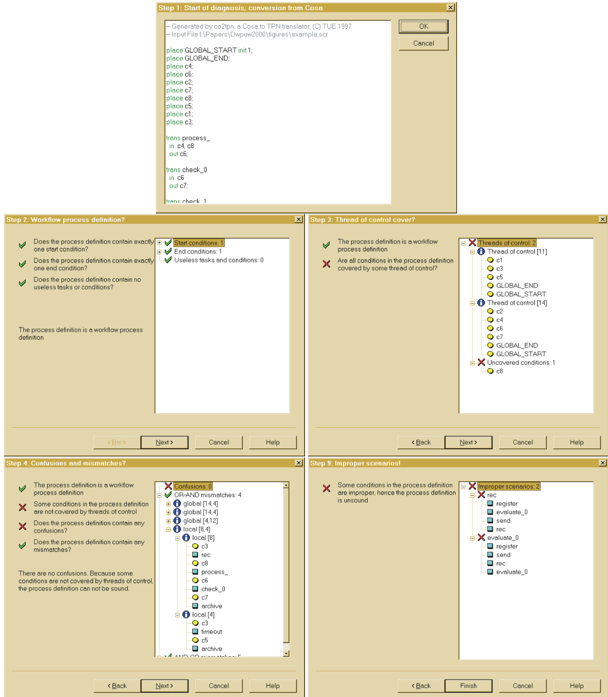
FIGURE 20. Example diagnosis, dialogs
