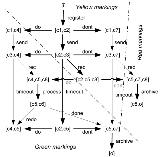
FIGURE 15. The RCG partitioned for unboundedness
