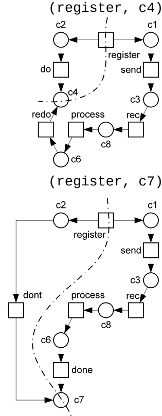
FIGURE 5. TP-handles in net N
