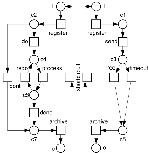
FIGURE 6. S-components of net N
