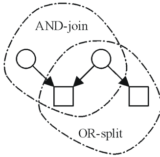
FIGURE 17. A non-free-choice cluster (confusion)
