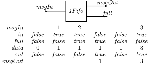
Figure 2. Sample behavior of a 1-place buffer
