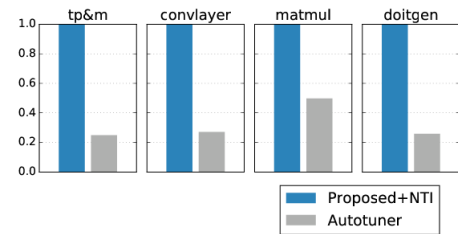
Figure 5. Throughput (1/s) relative to fastest implementation; autotuner ran for 1 day on Intel 5930K
