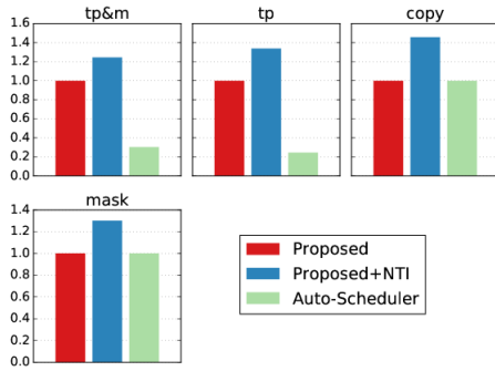
Figure 4. Intel platforms - Throughput (1/s) relative to fastest implementation (see Table 4)
