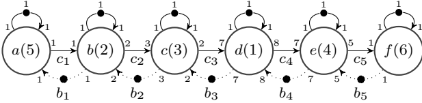
Fig. 3: The CSDF graph for a sample rate converter with additional storage constraints.
