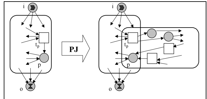
Figure 10. Inheritance-preserving transformation rule PJ.
