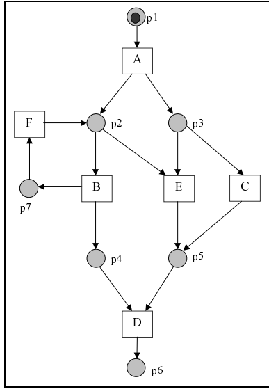
Figure 4. An incorrect workflow process definition.
