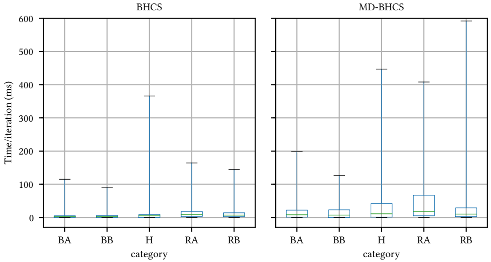
Fig. 7. Runtime per scheduling decision for BHCS and MD-BHCS (outliers included in whiskers).
