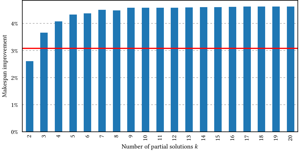
Fig. 4. Average makespan improvement of MD-BHCS (vertical blue bars) and BHCS (horizontal red line) over HCS.
