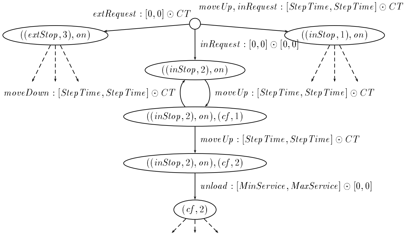
Fig. 3. Fragment of the Timed Transition System after Weaving.
