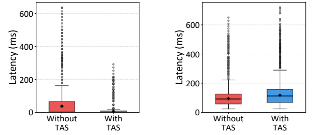
(a) Time-Critical latency with and without TAS. (b) Best-Effort latency with and without TAS.
