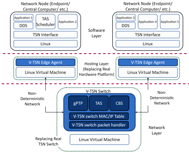
Fig. 1: The V-TSN overlay. Each endpoint and the switch run as software components on Linux virtual machines, interconnected over a general-purpose, non-deterministic network. The V-TSN switch replaces a physical TSN switch and implements gPTP synchronization, TAS, and CBS in software.
