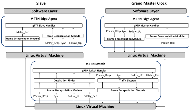
Fig. 3: Virtual gPTP synchronization in the V-TSN platform.
