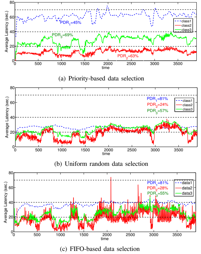
Fig. 4. The average latency of received data items from all nodes in each class generated at the same time and their average PDRs in setup 1.
