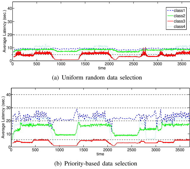
Fig. 7. The average latency of received data items for each class of nodes in COPD experiment setup.
