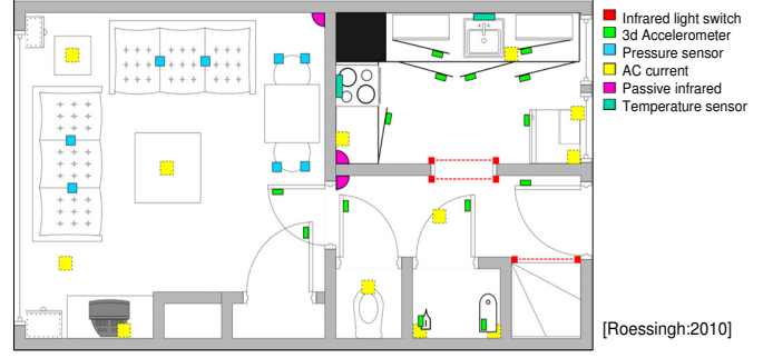
Fig. 6. The floor plan and node placement in the COPD experiment.
