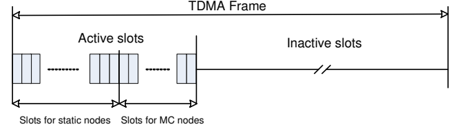
Fig. 1. The structure of a TDMA frame in the MCMAC protocol.
