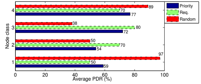
Fig. 8. The requested and achieved PDR values in COPD experiment setup.
