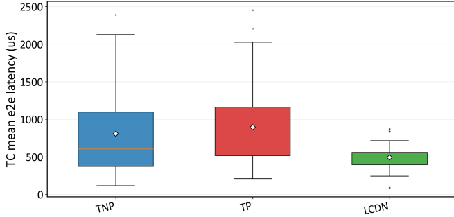
(c) Mean end-to-end latency of admitted TC flows (HERMES excluded for readability).
