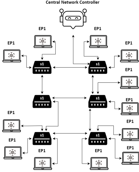
(a) Mesh topology.
