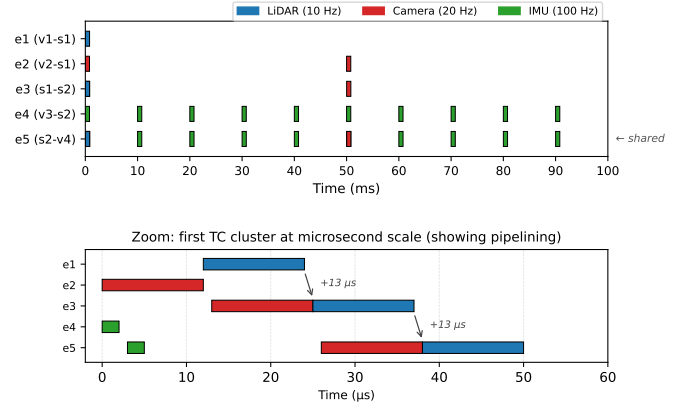
Fig. 2: TNP: collision-free placement of all 13 TC frames. Top: per-link timelines over one 100 ms cycle (schematic). Bottom: zoom into the first TC cluster at the microsecond scale.
