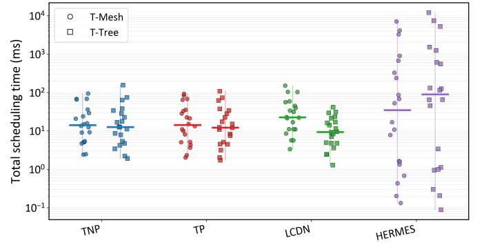
Fig. 10: Total scheduling time per method across all 20 scenarios on both topologies (log scale).
