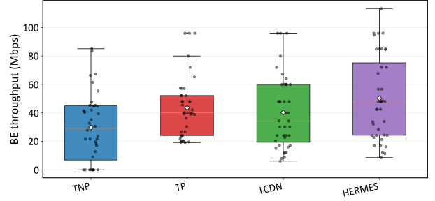
Fig. 12: Aggregate BE throughput across all 40 configurations.
