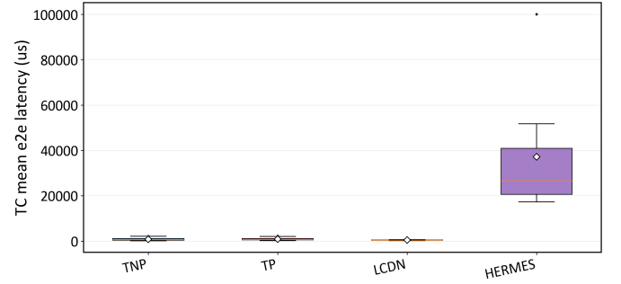
(b) Mean end-to-end latency of admitted TC flows across all 40 scenarios.
