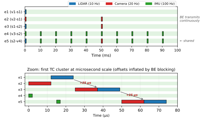
Fig. 4: TP: TC frame placement with offsets inflated by worst-case BE blocking. Top: per-link timelines over one 100 ms cycle (schematic). Bottom: zoom into the first TC cluster at the microsecond scale. The shaded background indicates BE traffic may transmit at any time outside the intervals occupied by TC frames.
