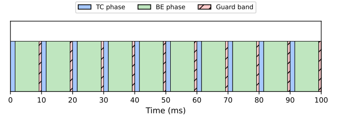
Fig. 3: TNP: visualization of the GCL cycle, enforced identically at every endpoint, with 10 TC phases, BE phases, and guard bands over one 100 ms cycle (schematic, not to scale).
