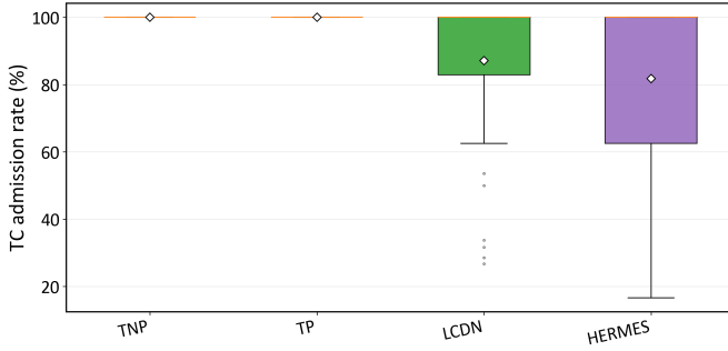
(a) TC admission rate across all 40 scenarios.
