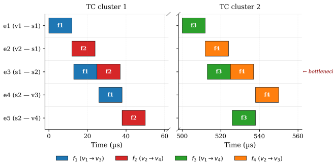
Fig. 5: Per-link occupancy after the TC Scheduling Agent places the four TC flows. The broken time axis displays the two TC clusters at a readable scale.
