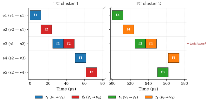
Fig. 7: Per-link occupancy under TP method.
