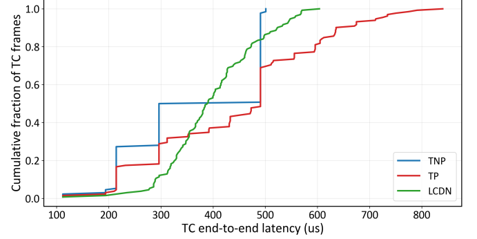
(d) CDF of per-frame TC end-to-end latency for scenario H2-B2 on the tree topology.
