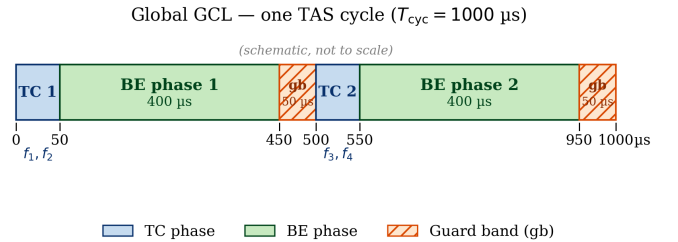
Fig. 6: The global GCL for the running example.
