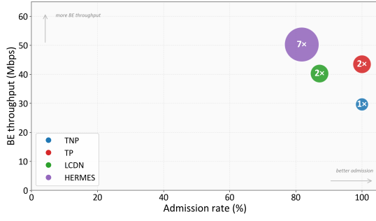
Fig. 13: Overall trade-off: mean TC admission rate vs. mean BE throughput. Circle size indicates estimated relative deployment cost.
