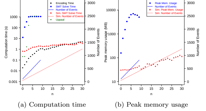
Fig. 5. The mean computation time, peak memory usage and number of events for \phi_{2,i} as a function of n .
