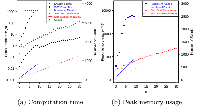
Fig. 6. The mean computation time, peak memory usage and number of events for \phi_3 as a function of n .
