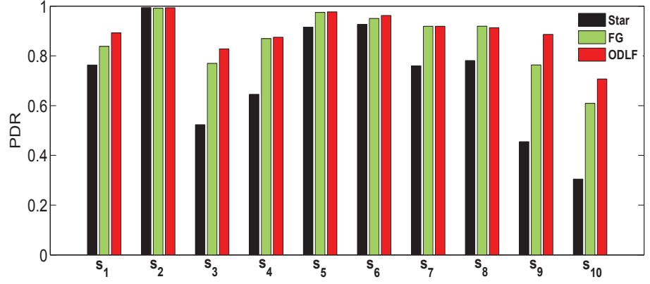
Fig. 7. Average PDR of nodes to the gateway over all experiments exploiting different protocols.
