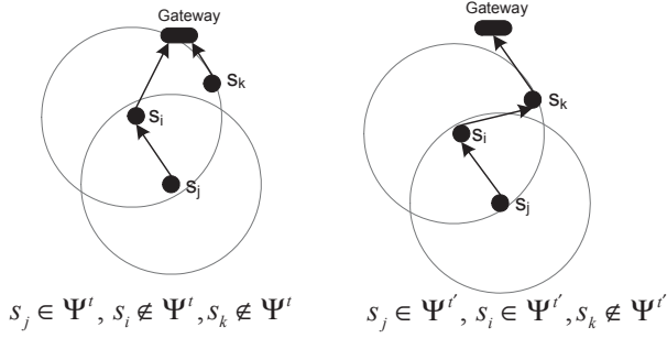
Fig. 5. An illustrative example of the on-demand forwarding mechanism.
