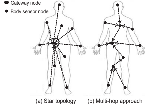
Fig. 1. Common approaches for intra-WBAN communication.
