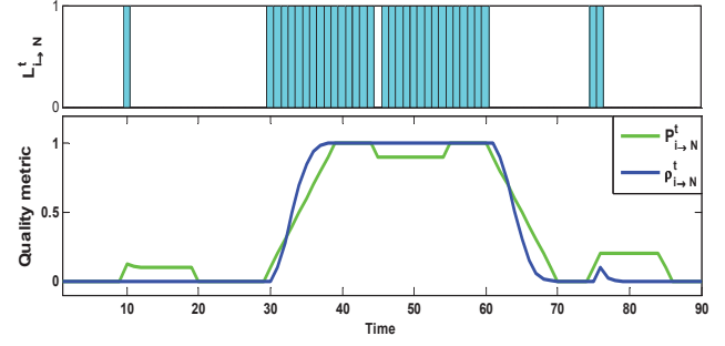
Fig. 4. Packet Reception Ratio (PRR) and the derived link quality metric for a sample link L_{i \rightarrow N} .
