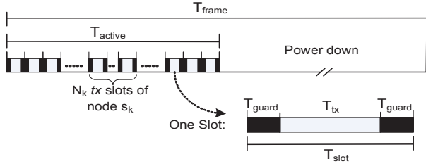
Fig. 2. The structure of a TDMA frame of the MAC protocol
