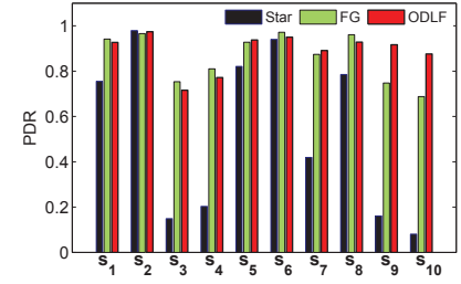
Fig. 9. PDR of different body sensor nodes to the gateway in an experiment with low quality links.
