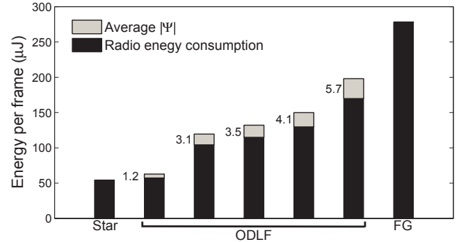
Fig. 10. Average energy consumption using ODLF protocol in experiments with different link quality, and the consumption in Star and FG protocols.
