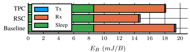
Fig. 4. The energy per byte with LPL for three configurations: Baseline with maximum transmission power and reception sensitivity, TPC with reduced transmission power, RSC with reduced sensitivity.
