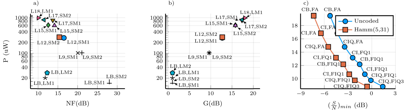
Fig. 2. The component characteristics. The analog estimation of power (P) vs. noise figure (NF), and signal gain (G) are shown in a) and b). The estimation of power consumption and minimum signal-to-noise ratio for coded and uncoded modes are shown in c).
