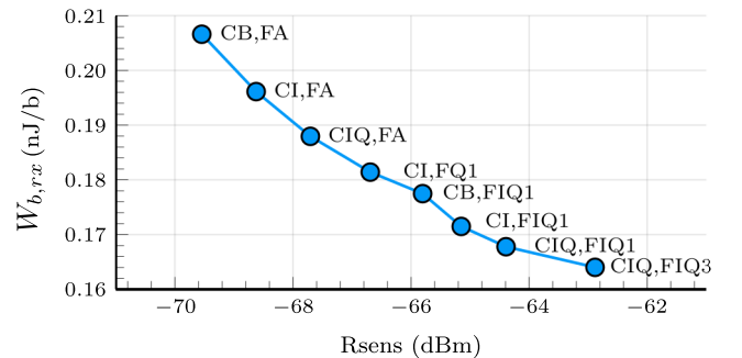
Fig. 6. The Pareto-optimal configurations in the lower sensitivity requirement region. The different ADB configurations yield significant energy savings.
