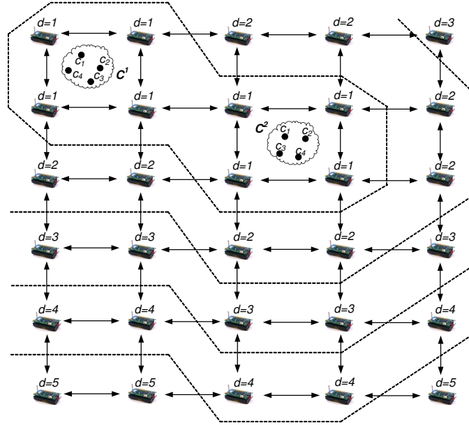
Fig. 6. Hop-distance estimation from the nearest cluster in a 6 \times 5 nodes static WSN with two mobile clusters, each containing four nodes. Regions with the same d values are pointed out. The regular deployment is only to illustrate the hop-distance concept. The MCMAC protocol does not assume such a deployment.
