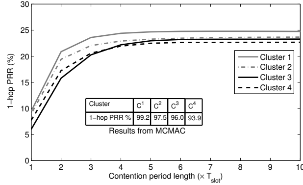
Fig. 15. The overall 1-hop PRR for mobile clusters in the M-LMAC protocol using various lengths of the contention period. The table in the figure shows the 1-hop PRR achieved in the experiments running the MCMAC protocol (taken from Table II).
