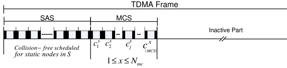
Fig. 3. A TDMA frame containing the SAS and MCS parts.
