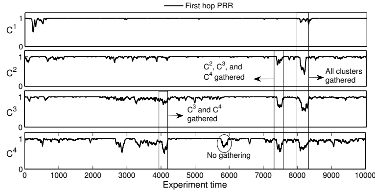
Fig. 13. 1-hop PRR of the mobile clusters over a sliding window of size 20 frames.
