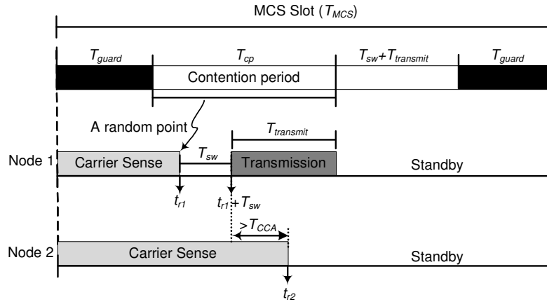
Fig. 4. The structure of a time slot prepared for performing CSMA in the MCS part of the frame.
