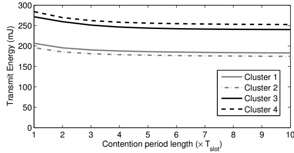
Fig. 16. Transmit energy consumption of mobile cluster nodes during the whole experiment, performing the M-LMAC protocol for various lengths of the contention period. The values are the average over the 4 nodes in each cluster. The transmit energy consumption of the mobile cluster nodes in MCMAC during the experiment is 70mJ.
