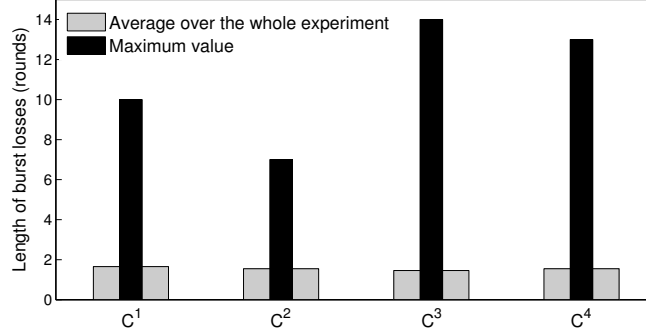
Fig. 12. The length of packet loss bursts averaged over all nodes in each mobile clusters and over the whole experiment time. The graph also shows the maximum length of bursts losses.
