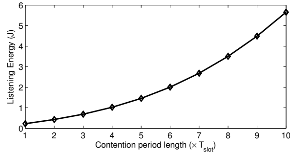
Fig. 17. Average energy consumption of static nodes for listening to mobile nodes during the whole experiment, performing the M-LMAC protocol for various lengths of the contention period. The average listening energy consumption of static nodes in an MCMAC experiment is 541mJ.
