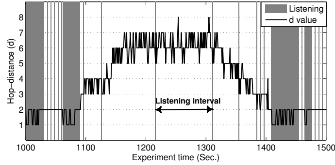
Fig. 7. The variations of the estimated hop-distance d in a duration of a real experiment for a sample static node and its decision about listening to the MCS part.
