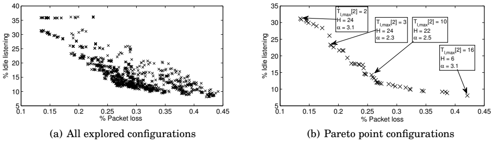
Fig. 9. Empirical exploration of the configuration space for listening scheduling mechanism.
