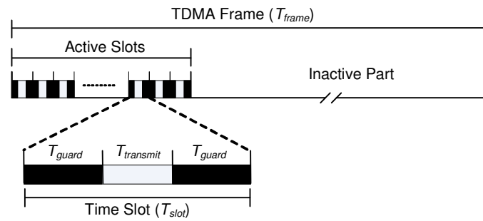
Fig. 2. The basic structure of the TDMA frames and time slots.
