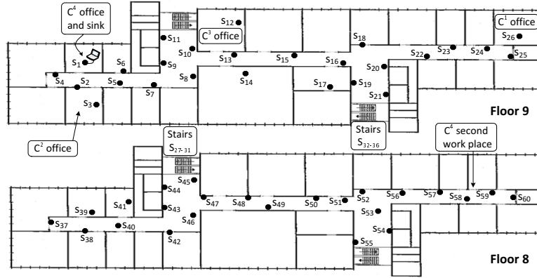
Fig. 10. Node deployment on two floors ( 8^{th} and 9^{th} ) of the EE department of TU/e.
