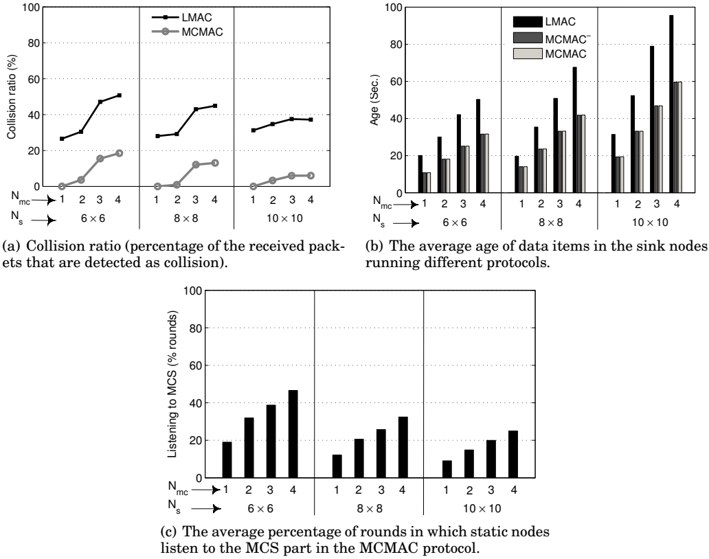
Fig. 18. Simulation results for different network setups and protocols.
