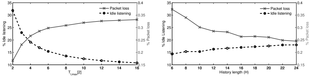
(a) Trade-off made by maximum size of listening interval. (b) Trade-off in terms of the averaging length ( H ).
