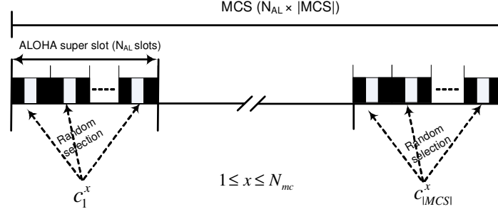
Fig. 5. The structure of a super slot prepared for performing slotted ALOHA in the MCS part of the frame.
