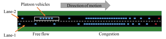
Figure 2: SUMO GUI – a five-vehicle platoon driving on a two lane road segment approaching a stop-and-go wave.
