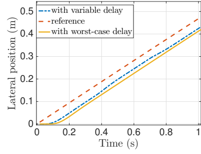
Fig. 7: Lateral position of the vehicle w.r.t. the road centre.
