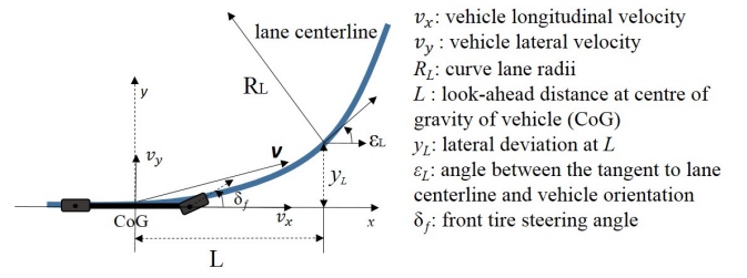
Fig. 6: Vision-based lateral control system derived from [15].
