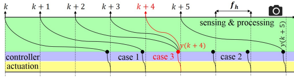
Fig. 5: Illustration of cases described in Section IV-B. The samples k+3 and k+4 have lower workloads and thus the latest output measurement y(k+4) is available within one f_h . Note that for case 2, the latest measurements are not available and thus u(k+i) is computed based on the MPC prediction model.
