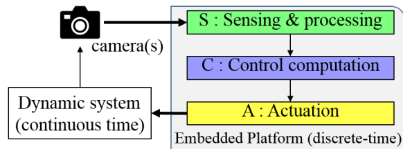
Fig. 1: An image-based control (IBC) system: block diagram
