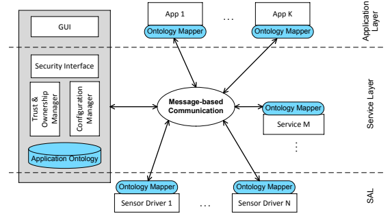
Figure 5: The architecture with decentralized data stores (local data stores are not shown).
