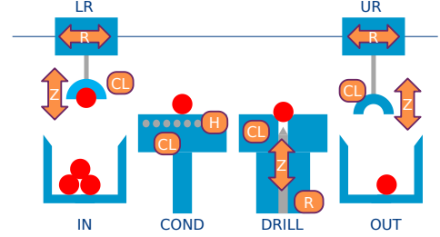
Fig. 7. Twilight manufacturing system [15].
