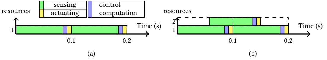
Fig. 1. Example resource configuration of image-based control. a) Sequential configuration. b) Pipelined configuration with two sensing cores.
