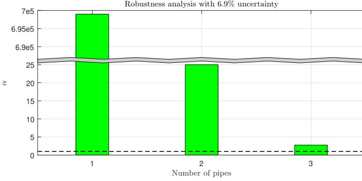
Fig. 10. Robustness analysis in the feasibility study
