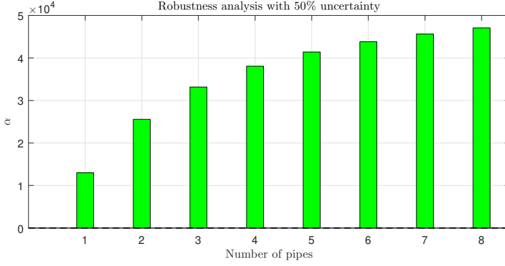
Fig. 6. Robustness analysis including the control design.
