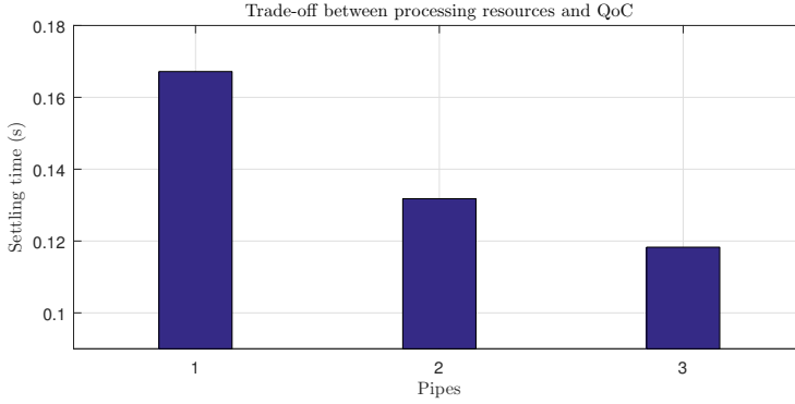
Fig. 9. Trade-off analysis without considering model uncertainties.
