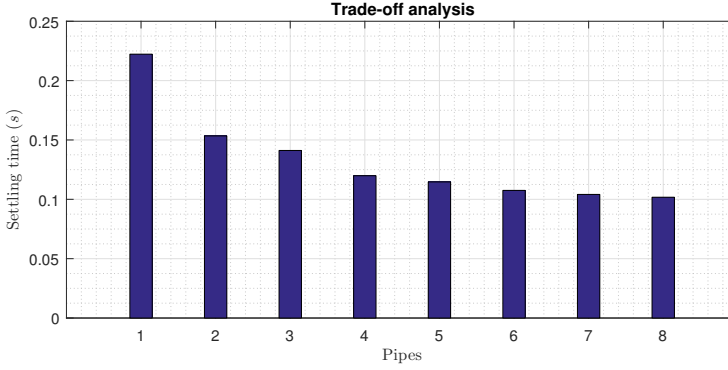
Fig. 3. Trade-off of the example of Section 3.1, without considering model uncertainties.
