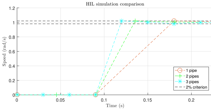
Fig. 12. Step responses comparison with different resource configurations using HIL simulation.
