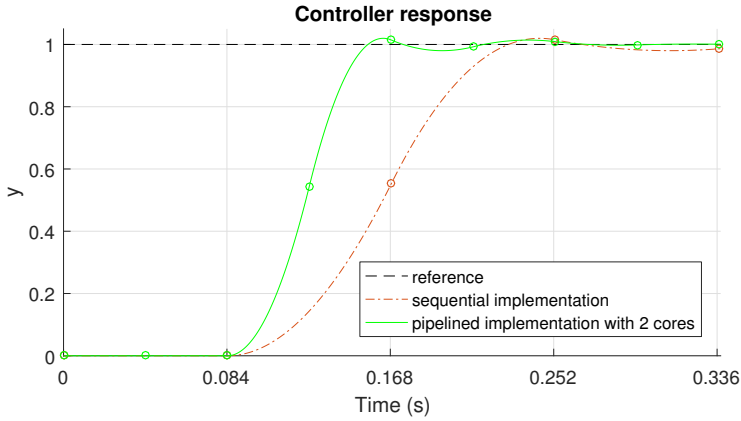
Fig. 2. Example of controller response with and without pipeline. The round markers denote multiples of the sampling period.
