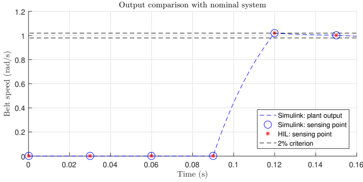
Fig. 11. Performance comparison 3 cores pipelined controller.
