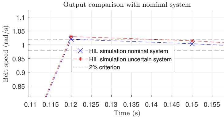
Fig. 13. Output of HIL simulation when the uncertain system is considered.
