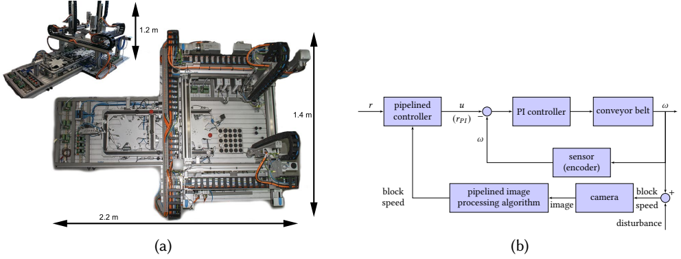
Fig. 7. Plant of feasibility study. (a) Assembly line xCPS. (b) Controller structure of one of the belts.
